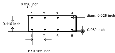
Figure 3: Transformer foot print.
