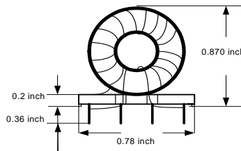
Figure 2: Physical Dimensions in inch.
