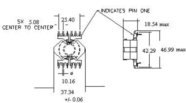
Figure 2: Physical Dimensions in mm.
