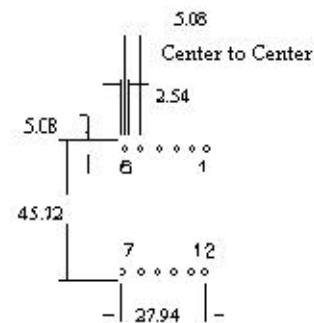
Figure 3: Transformer foot print.
