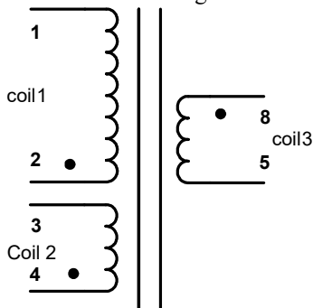
Figure 1: Schematic Diagram
